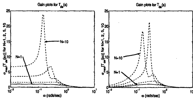
Figure 8: \bar{\sigma}(\bar{T}_{de}(j\omega)) for N = 1, 2, 5, 10 . Left: Bidirectional strategy: K_f(s) with no poles at s = 0 . Right: Bidirectional strategy: K_f(s) with a pole at s = 0 .
