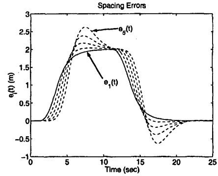
Figure 5: Time domain plots of spacing errors with the predecessor following strategy.
