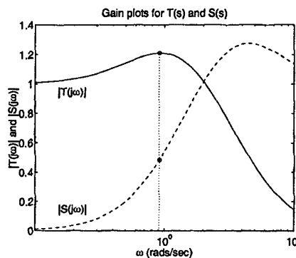
Figure 3: Plots of |T(j\omega)| and |S(j\omega)|
