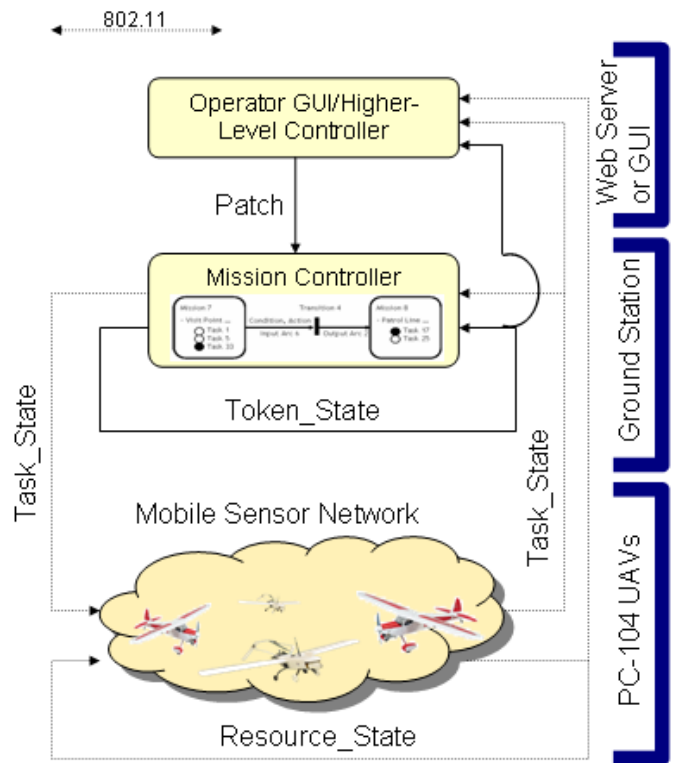
Fig. 1. Feedback Control of Sensor Networks
